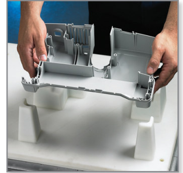
Image 1: Oreck uses direct digital manufacturing to produce custom assembly pallets. During assembly, a vacuum top cover is placed into the pallet upside down.
