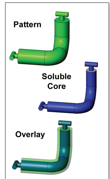
Figure 2: STLs of the pattern and soluble core for a radiator hose. The overlay shows how they are combined to form the internal passage.
